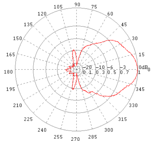
H-Ebene / H-Plane 2.8 GHz
