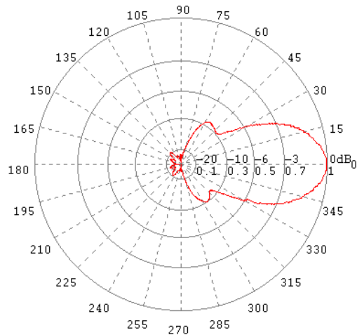
E-Ebene / E-Plane 2.0 GHz
