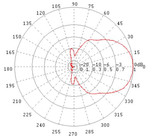
H-Ebene / H-Plane 2.0 GHz
