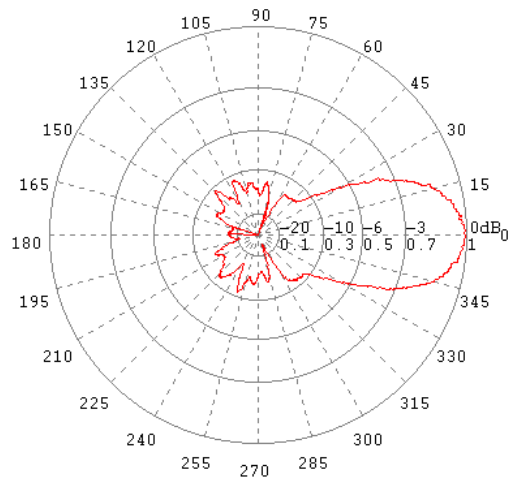
E-Ebene / E-Plane 2.8 GHz
