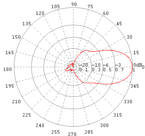
E-Ebene / E-Plane 1000 MHz
