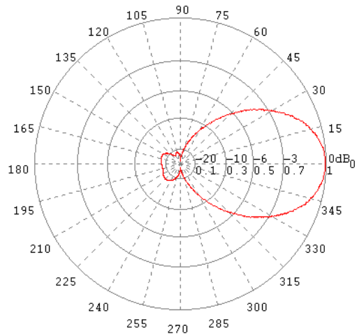
E-Ebene / E-Plane 500 MHz
