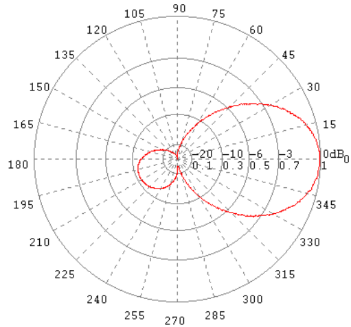
E-Ebene / E-Plane 230 MHz
