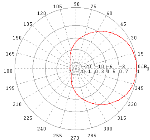
H-Ebene / H-Plane 500 MHz
